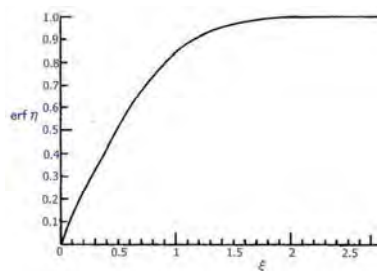
誤差関数 \operatorname{erf} \eta = (2/\pi^{1/2}) \int_0^{\eta} e^{-at^{1/2}} d\xi
